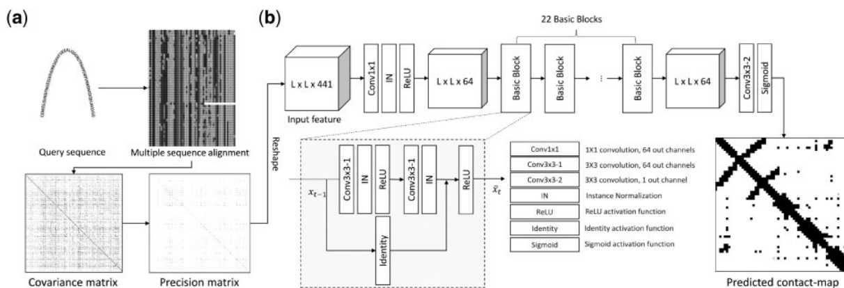
Fig. 1. Flowchart of ResPRE. (a) Process of precision-matrix based feature collection. (b) Block diagram of deep residual neural network architecture
